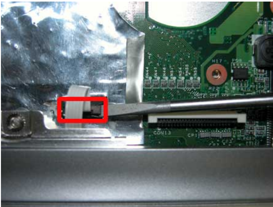
Fig. 26 Touch Pad connection
